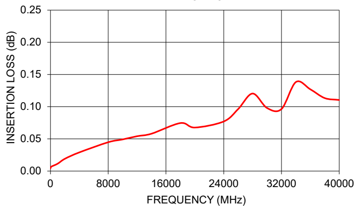
KMNMMD-24MNMMD+ INSERTION LOSS
