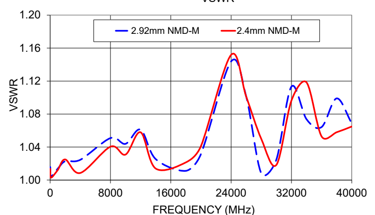
KMNMMD-24MNMMD+ VSWR
