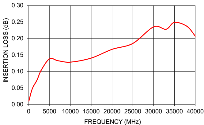
KMR-24F+ INSERTION LOSS
