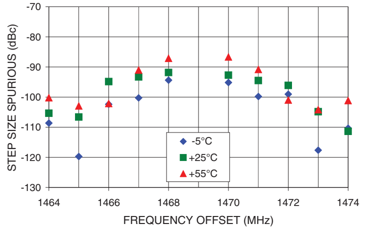
STEP SIZE SPURIOUS Vs FREQ. OFFSET @ Fcar = 1469MHz
