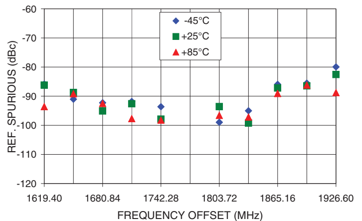
REFERENCE SPURIOUS Vs FREQ. OFFSET @ Fcar = 1773MHz
