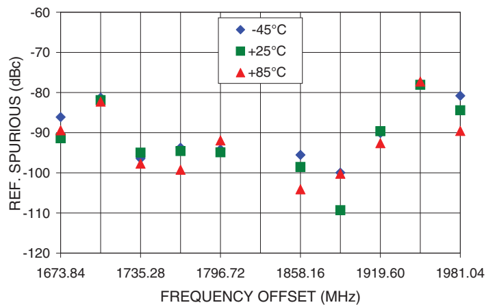
REFERENCE SPURIOUS Vs FREQ. OFFSET @ Fcar = 1827.44MHz
