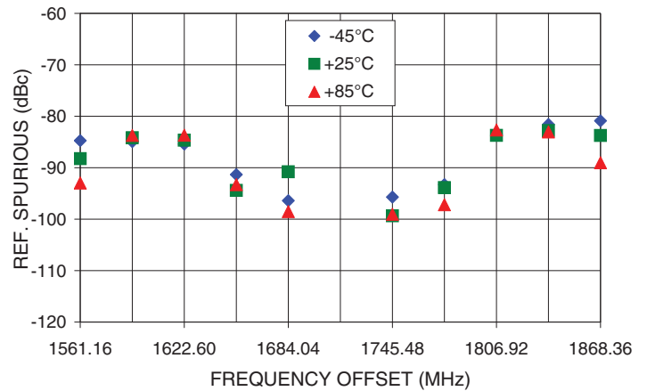
REFERENCE SPURIOUS Vs FREQ. OFFSET @ Fcar = 1714.76MHz
