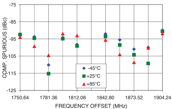
COMPARISON SPURIOUS Vs FREQ. OFFSET @ Fcar = 1827.44MHz
