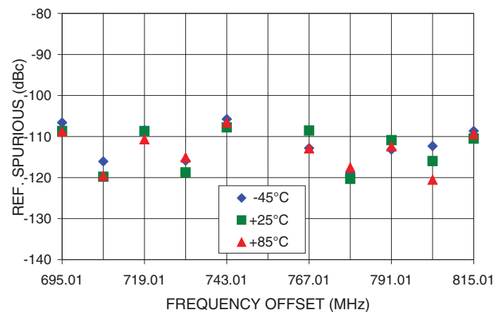
REFERENCE SPURIOUS Vs FREQ. OFFSET @ Fcar = 755.01MHz
