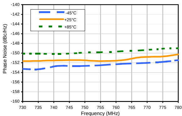
Phase Noise @ 1 MHz offset
