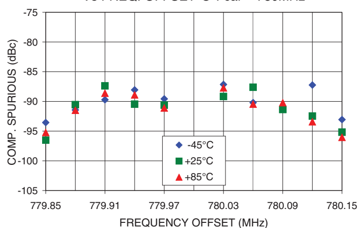
COMPARISON SPURIOUS Vs FREQ. OFFSET @ Fcar = 780MHz
