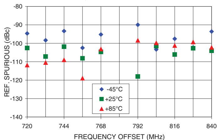
REFERENCE SPURIOUS Vs FREQ. OFFSET @ Fcar = 780MHz
