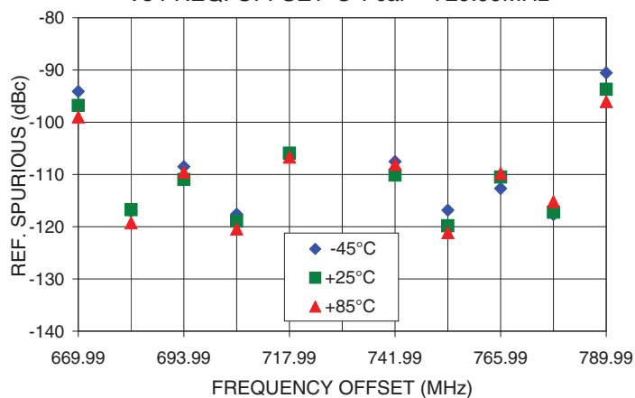
REFERENCE SPURIOUS Vs FREQ. OFFSET @ Fcar = 729.99MHz
