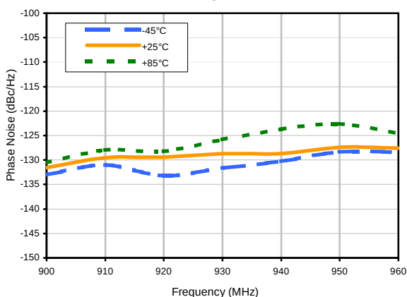
Phase Noise @ 100 kHz offset
