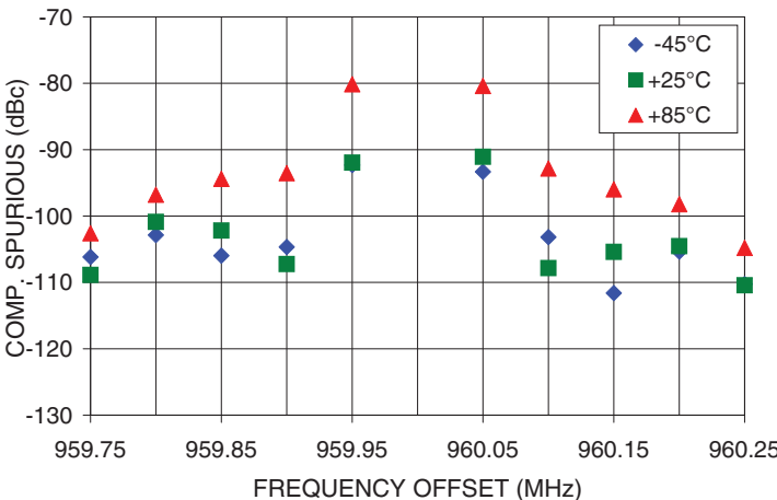
COMPARISON SPURIOUS Vs FREQ. OFFSET @ Fcar = 960MHz
