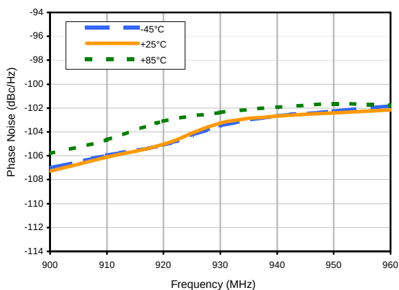
Phase Noise @ 10 kHz offset
