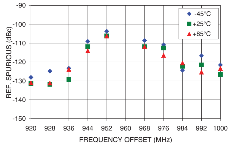
REFERENCE SPURIOUS Vs FREQ. OFFSET @ Fcar = 960MHz
