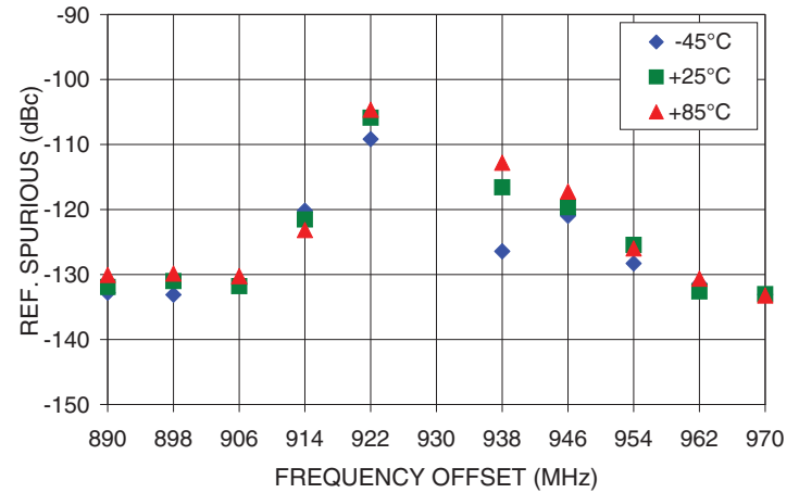
REFERENCE SPURIOUS Vs FREQ. OFFSET @ Fcar = 930MHz
