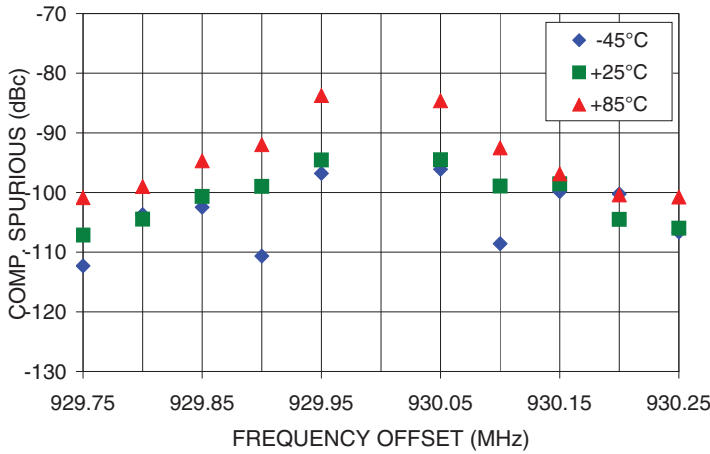
COMPARISON SPURIOUS Vs FREQ. OFFSET @ Fcar = 930MHz
