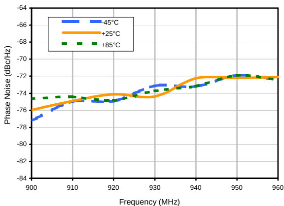
Phase Noise @ 1 kHz offset
