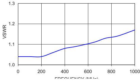
LAT-30+ VSWR
