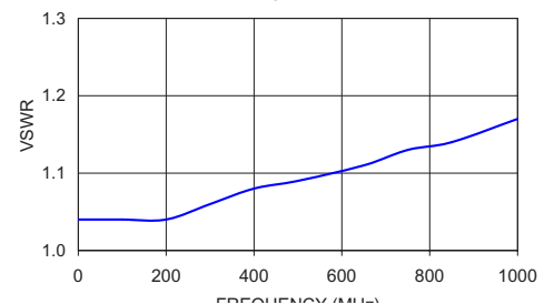
LAT-30+ VSWR
