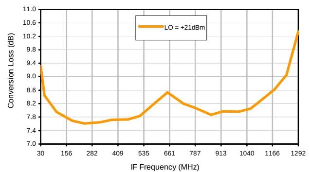
Conversion Loss vs. IF @ RF=2200.1MHz
