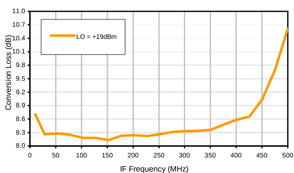
Conversion Loss vs. IF @ RF=1634.1MHz
