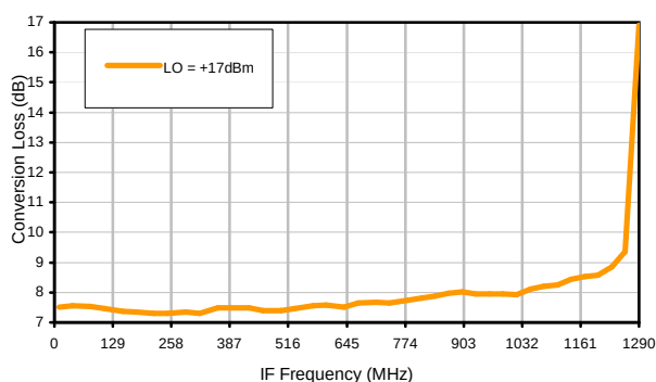
Conversion Loss vs. IF @ RF=1300.1MHz
