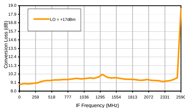
Conversion Loss vs. IF @ RF=2600.1001MHz
