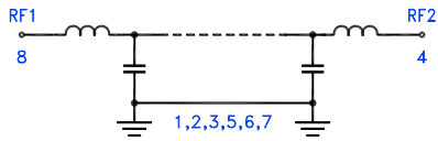
Figure 1. LFCG-2250+ Functional Diagram
