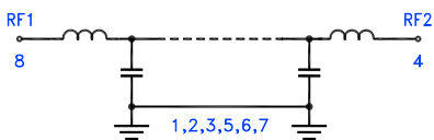
Figure 1. LFCG-2850+ Functional Diagram
