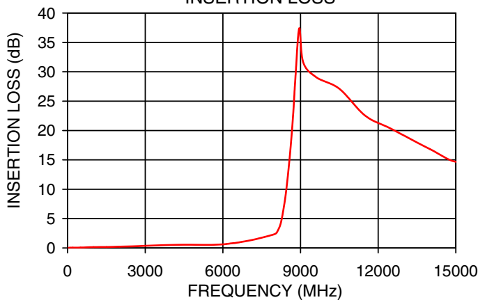
LFCN-7200+ INSERTION LOSS
