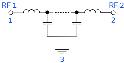
Figure 1. LFCV-2702+ Functional Diagram
