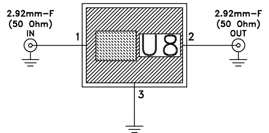
Schematic diagram
