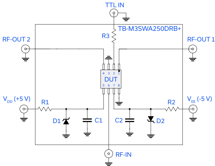
Figure 1. M3SWA-2-50DRB+ Characterization &amp; Application Circuit
