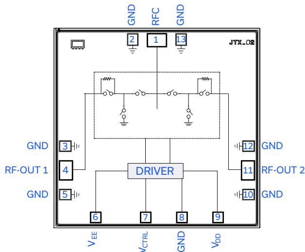
Figure 1. M3SWA2-34DR-D+ Functional Diagram
