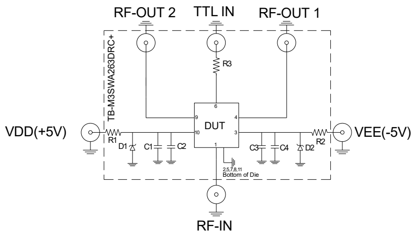
Figure 1. Characterization & Application Circuit
