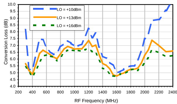
Conversion Loss vs. LO @ RF=1800.1 MHz
