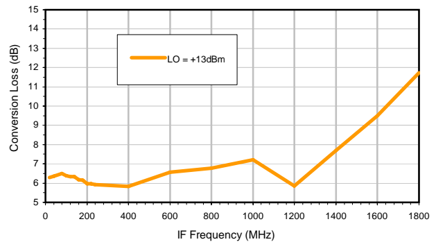
Conversion Loss vs. IF @ RF=4200.1 MHz
