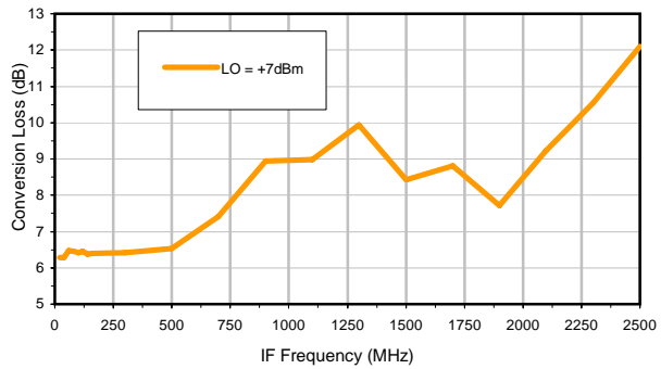
Conversion Loss vs. IF @ RF=6000.1 MHz
