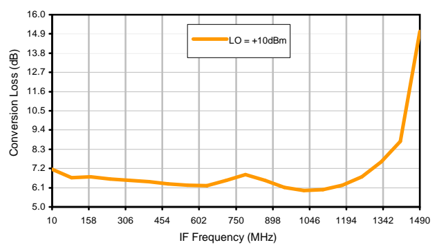
Conversion Loss vs. IF @ RF=3610.1MHz
