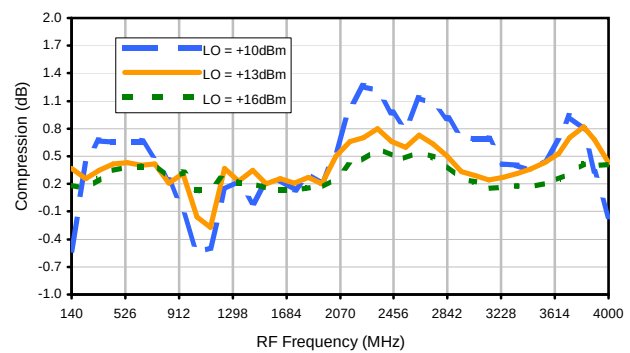
Compression @ RF IN=+9dBm
