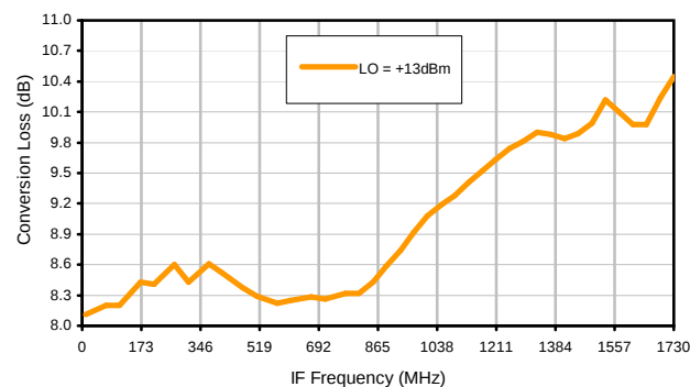
Conversion Loss vs. IF @ RF=3510.1MHz
