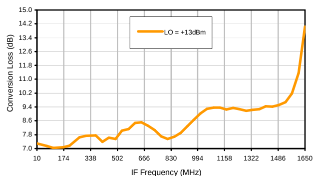
Conversion Loss vs. IF @ RF=1760.1MHz
