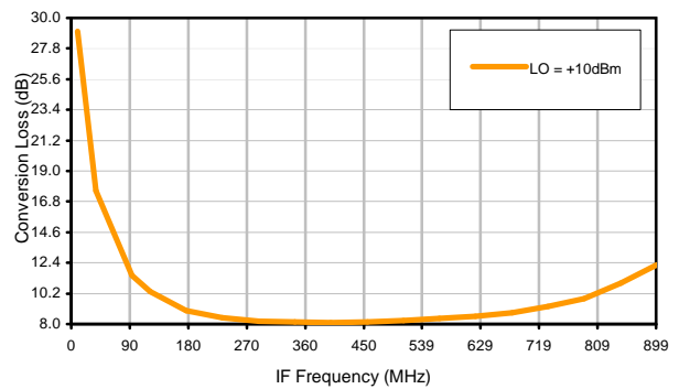
Conversion Loss vs. IF @ RF=3600MHz
