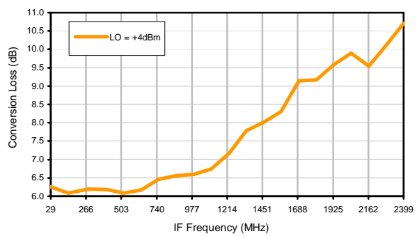
Conversion Loss vs. IF @ RF=12010.09MHz
