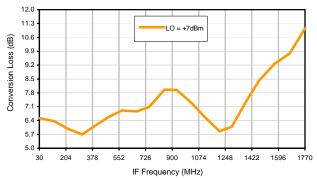
Conversion Loss vs. IF @ RF=4210.1MHz
