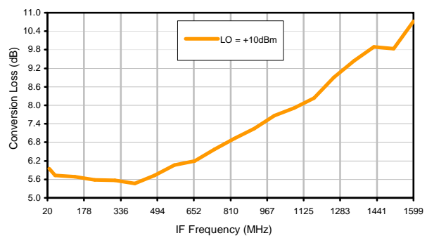
Conversion Loss vs. IF @ RF=8010.1MHz
