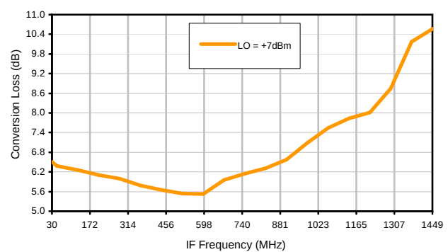
Conversion Loss vs. IF @ RF=8510.09MHz
