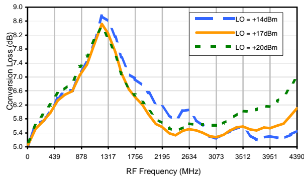
Conversion Loss vs. LO @ RF=1630.1MHz
