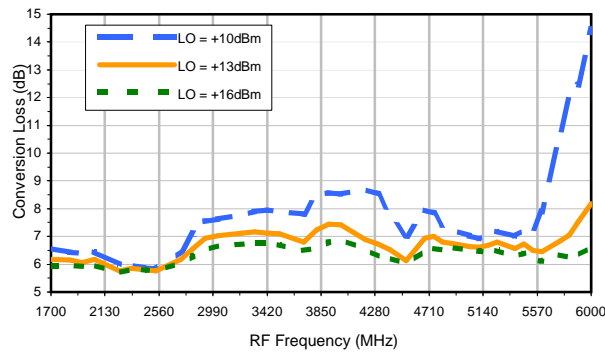
Conversion Loss vs. LO @ RF=3850 MHz
