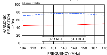
MIQC-176M HARMONIC REJECTION (LSB)
