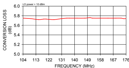
MIQC-176M CONVERSION LOSS
