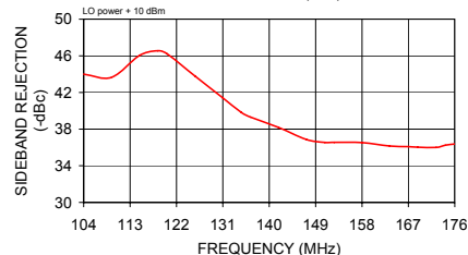
MIQC-176M SIDE BAND REJECTION (LSB)
