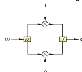
I&amp;Q modulation block diagram
