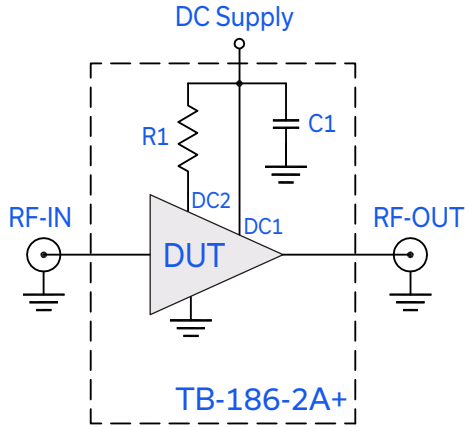
Fig 1. Block Diagram of Test Circuit used for characterization. (Die packaged in 3x3 mm 8-Lead QFN-Style Package and soldered on Mini-Circuits Characterization test board TB-186-2A+) Gain, Return Loss, Output Power at 1 dB Compression (P1dB), Output IP3 (OIP3) and Noise Figure measured using Agilent's N5242A PNA-X microwave network analyzer.
