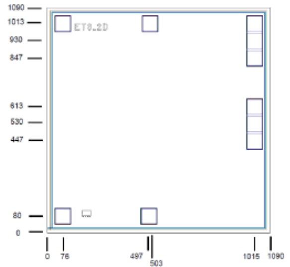
Fig 4. Bonding Pad Positions
