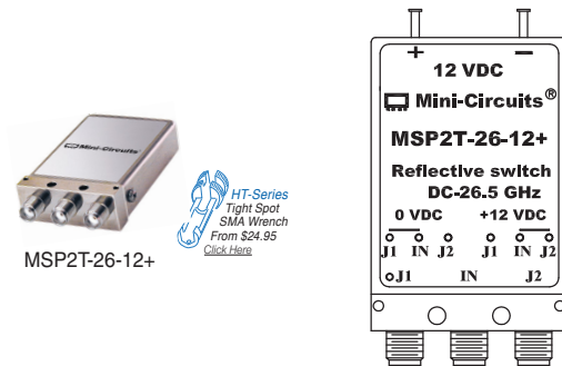
Marking Drawing
