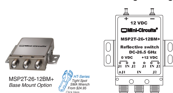
Marking Drawing
