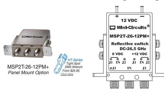
Marking Drawing
