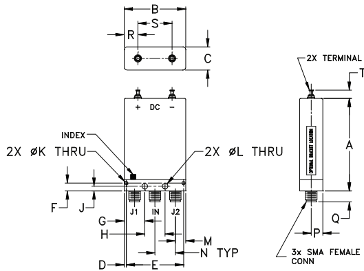
Outline Dimensions (inch)
