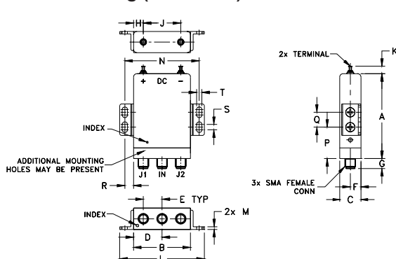
Outline Dimensions (inch)
