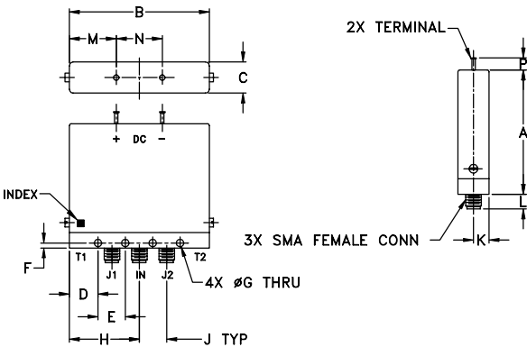
Outline Dimensions (inch mm)
