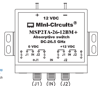
Marking Drawing
