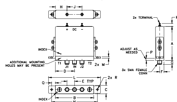
Outline Dimensions (inch/mm)
