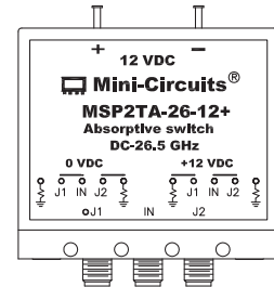
Marking Drawing
