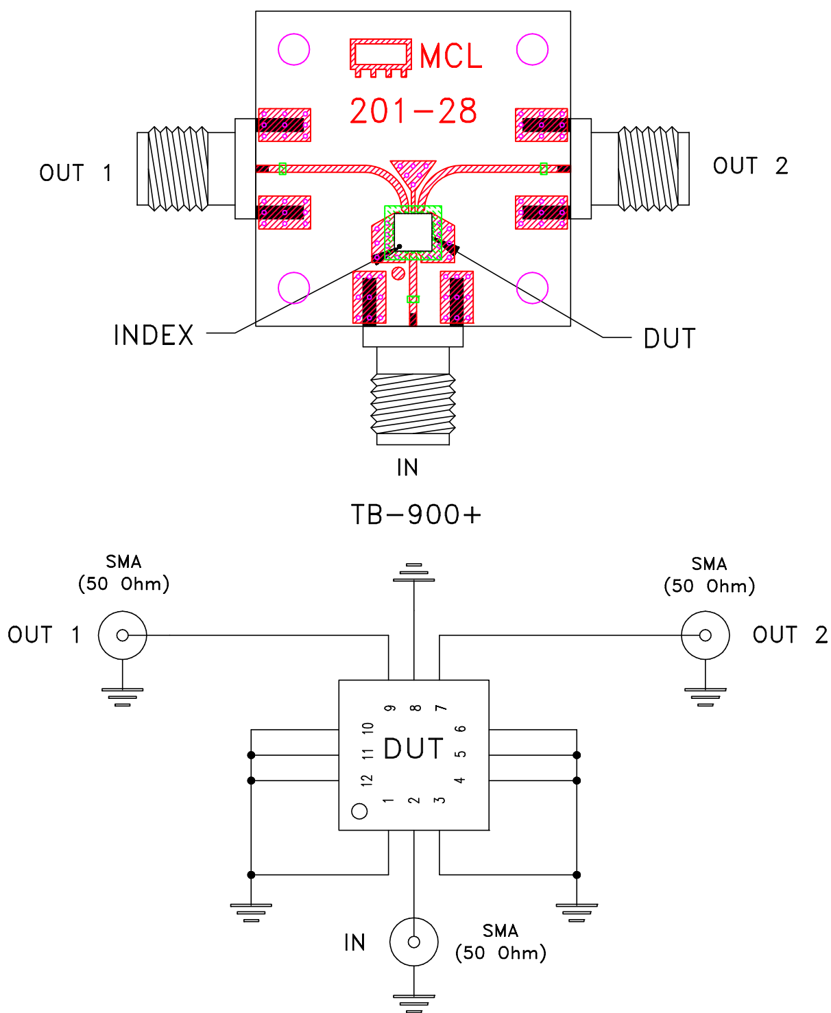
Schematic Diagram
