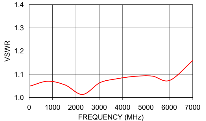
PAT-2+ VSWR
