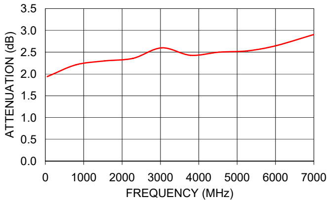
PAT-2+ ATTENUATION
