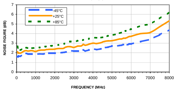
NOISE FIGURE vs. FREQUENCY & TEMPERATURE Vd = 3.3V
