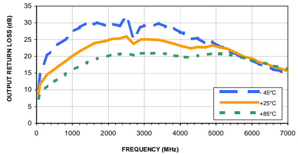
OUTPUT RETURN LOSS vs. FREQUENCY & TEMPERATURE Vd = 5V, Rbias=7.5K ohms
