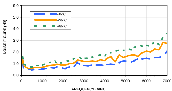
NOISE FIGURE vs. FREQUENCY & TEMPERATURE
