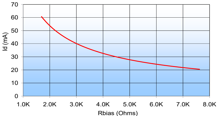
Typical Current ( I_d ) as a function of R_{bias} ( V_d = 5V )
