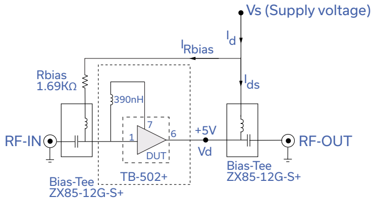
Fig 1. Block Diagram of Test Circuit used for characterization. (DUT soldered on Mini-Circuits Characterization Test Board TB-502+) Gain, Output power at 1dB compression (P1dB), Output IP3 (OIP3) and Noise Figure measured using Agilent's N5242A PNA-X Microwave network analyzer.
