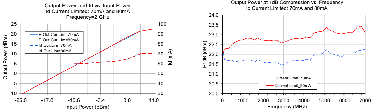
Fig 2. Output Power and Id vs. Input Power and Frequency. Performance measured on Mini-Circuits Characterization test board TB-502+. See Characterization Test Circuit (Fig. 1) Measurements performed with current (Id) limited as noted.
