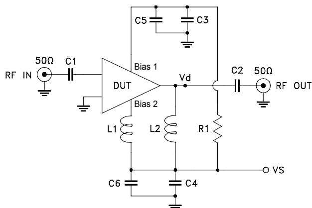
Component Description DUT PMA-545G1-D+ Die C1, C2, C5, C6 100 pF C3, C4 1 \mu F R1 0 \Omega L1 36 nH L2 47 nH
