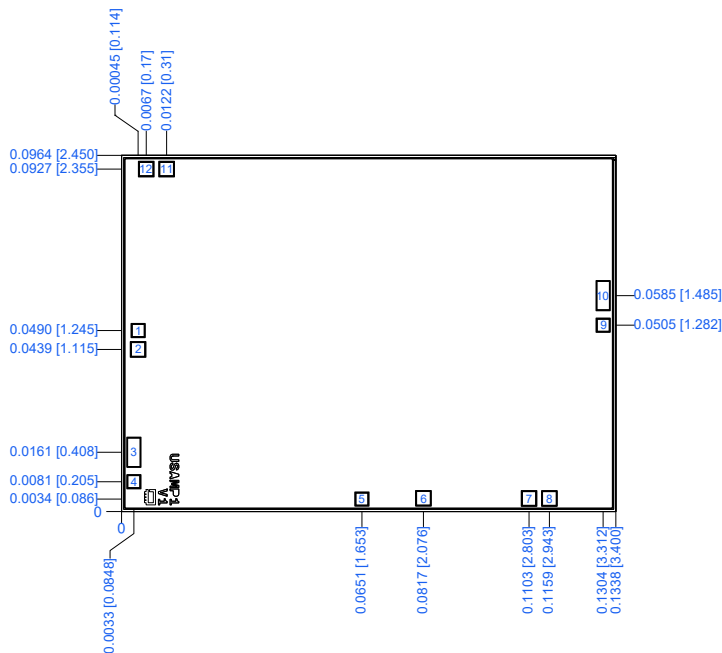
Figure 2. PMA5-83-2W-D+ Outline Drawing.
