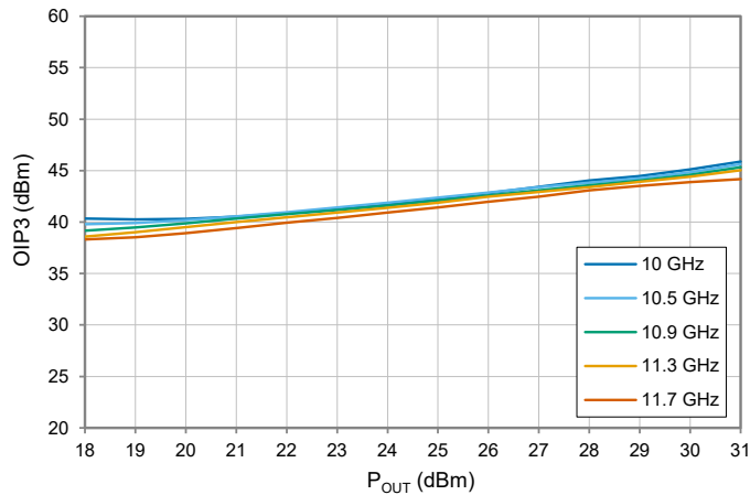
OIP3 vs. P_{OUT} /TONE V_{DD} = +8\text{ V} , TONE SPACING = 5 MHz, TEMPERATURE = +25°C
