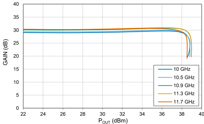
AM - AM V_{DD} = +8\text{ V} , TEMPERATURE = +25°C
