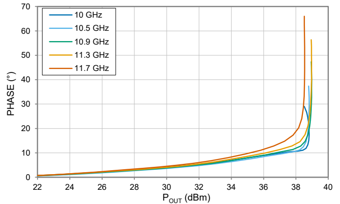
AM - PM V_{DD} = +8\text{ V} , TEMPERATURE = +25°C
