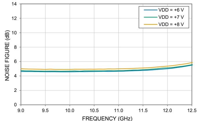
NOISE FIGURE vs. DEVICE VOLTAGE TEMPERATURE = +25°C
