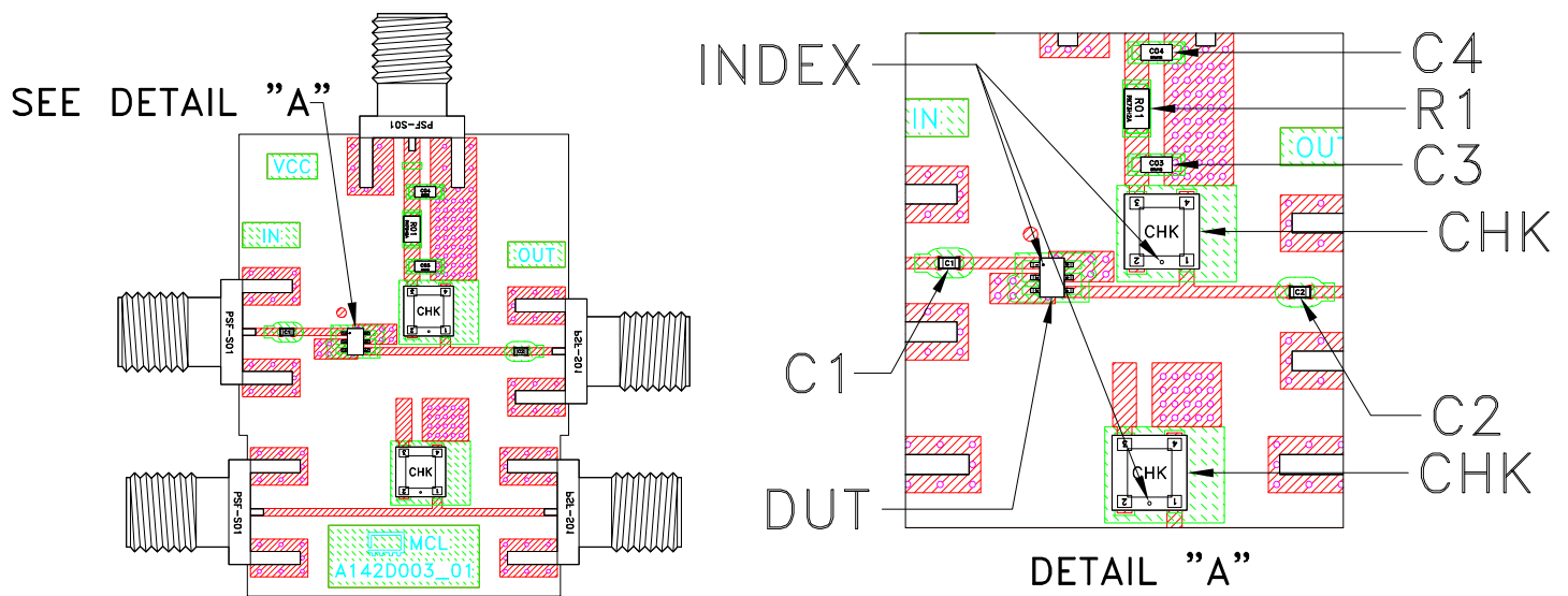
LOCATION OF COMPONENTS ON THE PCB (SCALE 1.5:1)
