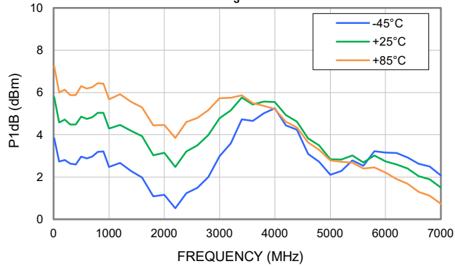
P1dB vs. TEMPERATURE, V_S = +5 V
