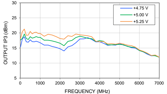
OUTPUT IP3 vs. V_S , P_{OUT} = -8 dBm/TONE, TEMPERATURE = +25°C
