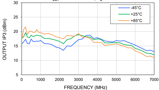
OUTPUT IP3 vs. TEMPERATURE, P_{OUT} = -8 dBm/TONE, V_S = +5 V
