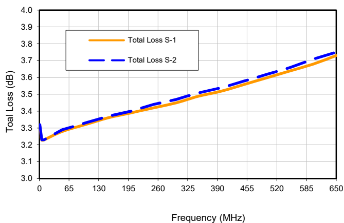
Total Loss
