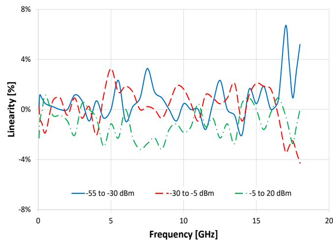
Linearity vs. Frequency
