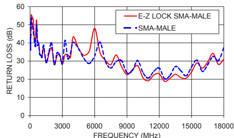
QBL1MSMQ-SM+ RETURN LOSS
