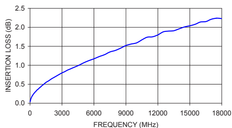
QBL1MSMQ-SM+ INSERTION LOSS
